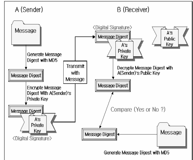
Figure 1. Basic Flow Chart of Digital Signature
