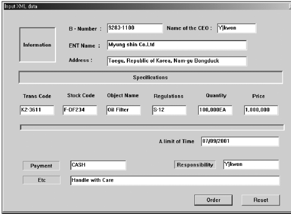
Figure 7. Delivery data input screen
